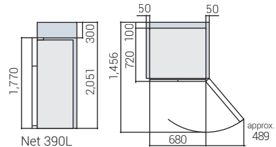
Net 390L □: Space required for ventilation.
